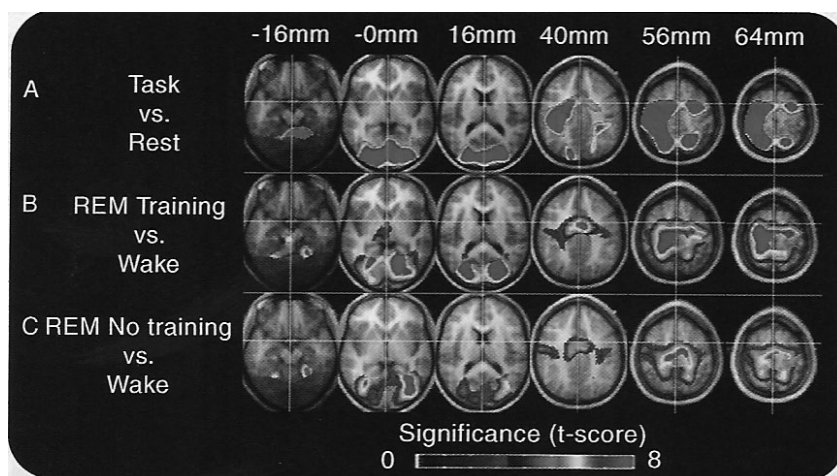
Fig. 5. Task-dependent reactivation of human brain activity during REM sleep. Statistical activation maps of different experimental contrasts. Maps are displayed at six different brain levels (from 16 mm below to 64 mm above the bicommissural plane), superimposed on the average MRI image of subjects. All maps are thresholded at P < 0.01 (uncorrected), except for (A), which is thresholded at voxel-level-corrected P < 0.05 (A) Brain regions activated during daytime performance of the motor skill task (Task versus Rest). (B) Brain regions activated during subsequent REM sleep in subjects that received daytime training (REM Sleep Training versus Wake). Note considerable overlap with daytime task-dependent activity patterns. (C) Brain regions activated during REM sleep in subjects who did not receive any daytime training (REM Sleep No Training versus Wake). (From Maquet P, Laureys S, Peigneux P, et al. Experience-dependent changes in cerebral activation during human REM sleep. Nat Neurosci 2000;3(8):831-6; with permission.)
